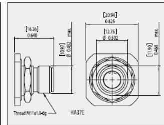
HA37E Jam Nut Fixing Dummy Receptacle
