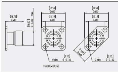
HA35E 2 Hole Dummy Receptacle / HA30E 4 hole Dummy Receptacle
