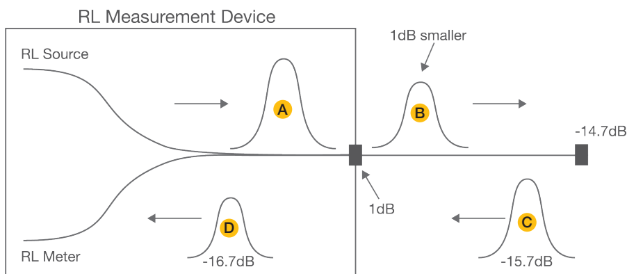
Figure 1: The optical signal travels twice along the same path; once in the forward direction and once in the reverse direction.
